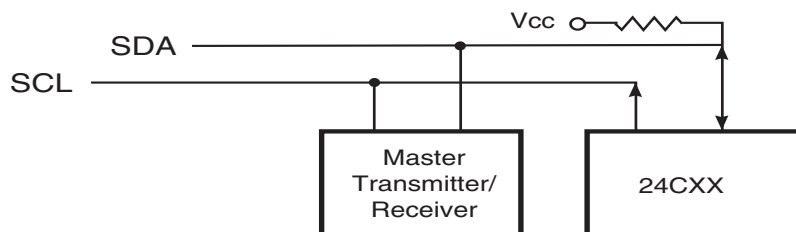
Figure 1. Typical System Bus Configuration
