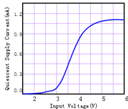
Fig2: Quiescent Supply Current VS Input Voltage
