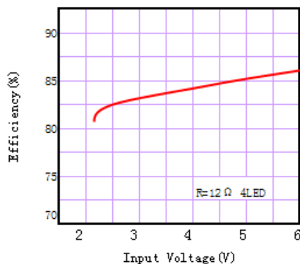
Fig3: Efficiency VS Input Voltage
