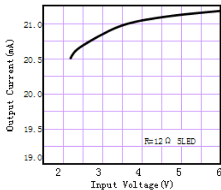
Fig1: Output Current VS Input Voltage
