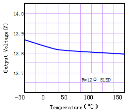
Fig4: Temperature VS Output Voltage
