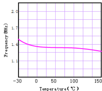
Fig4: Temperature VS Frequency
