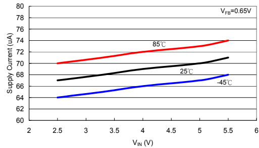
Line Regulation
