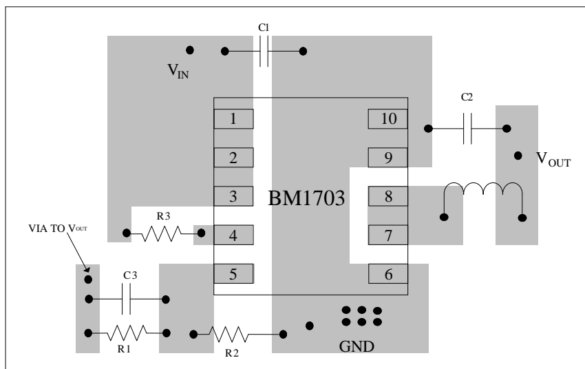
Suggested Layout for MSOP-10L
