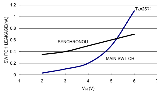
SWITCH LEAKAGE vs. INPUT VOLTAGE
